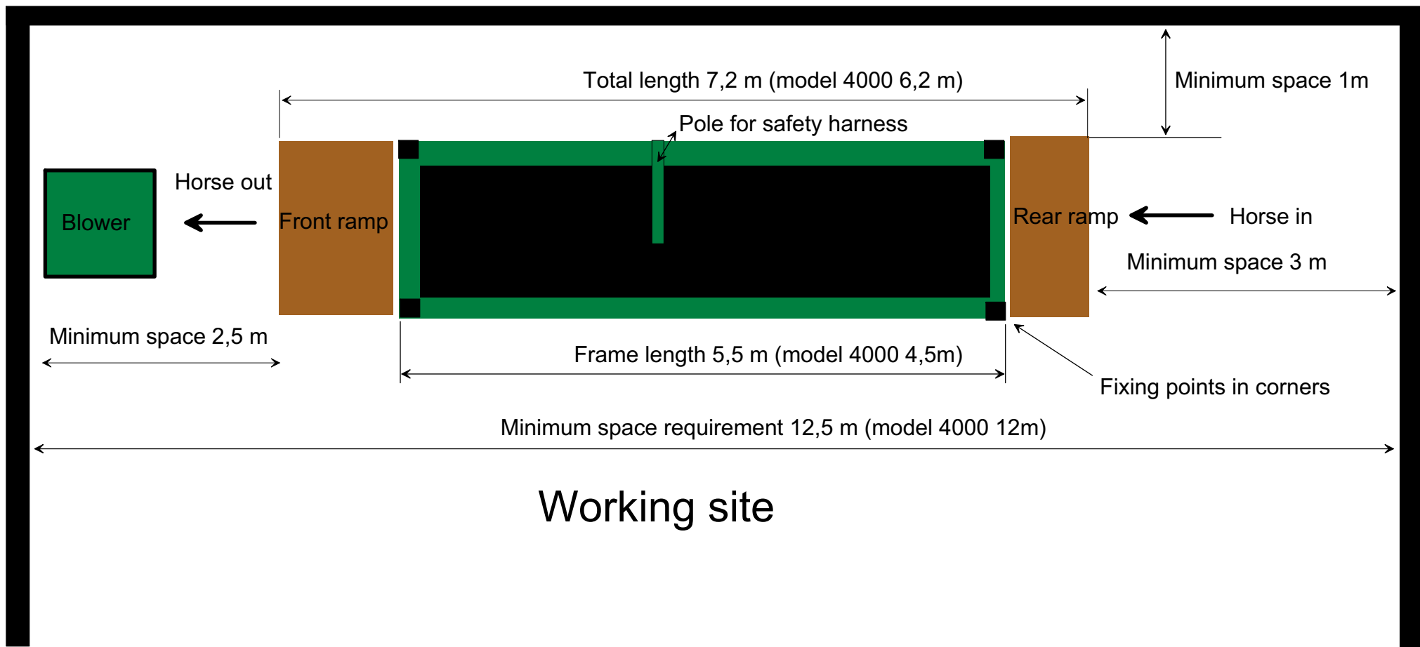
Haico treadmill model 5000 and 4000 space requirement
